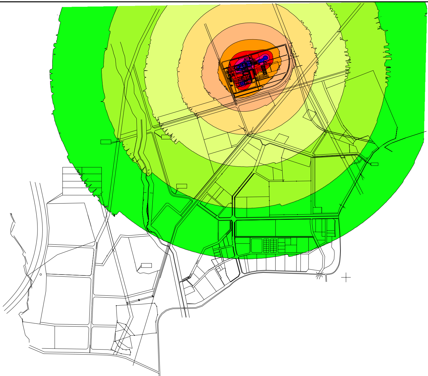
PROPOSED ADVANCED MATERIALS PLANT Normal Night-time Operation - Wind from all Direction LAeq Noise Level Contours to Surrounding Areas
